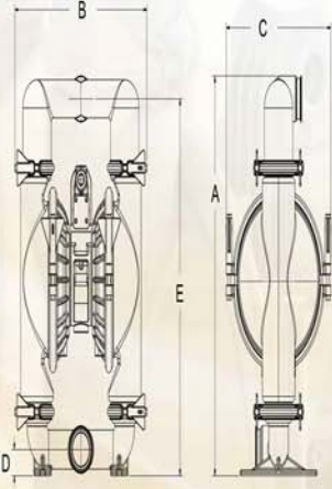
FDA Dimensional Drawings
